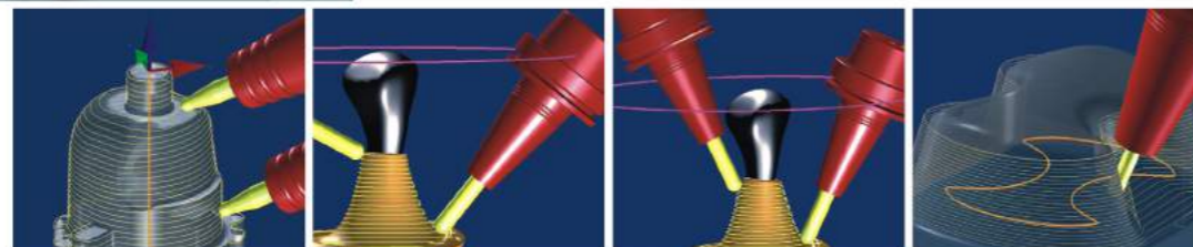
Tool axis facing towards Z-Axis.
